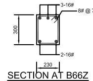
SECTION AT B66Z
