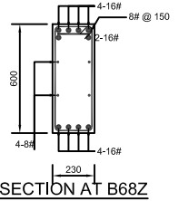
SECTION AT B68Z
