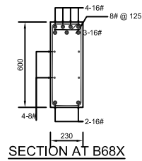
SECTION AT B68X
