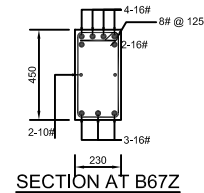
SECTION AT B67Z
