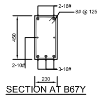
SECTION AT B67Y
