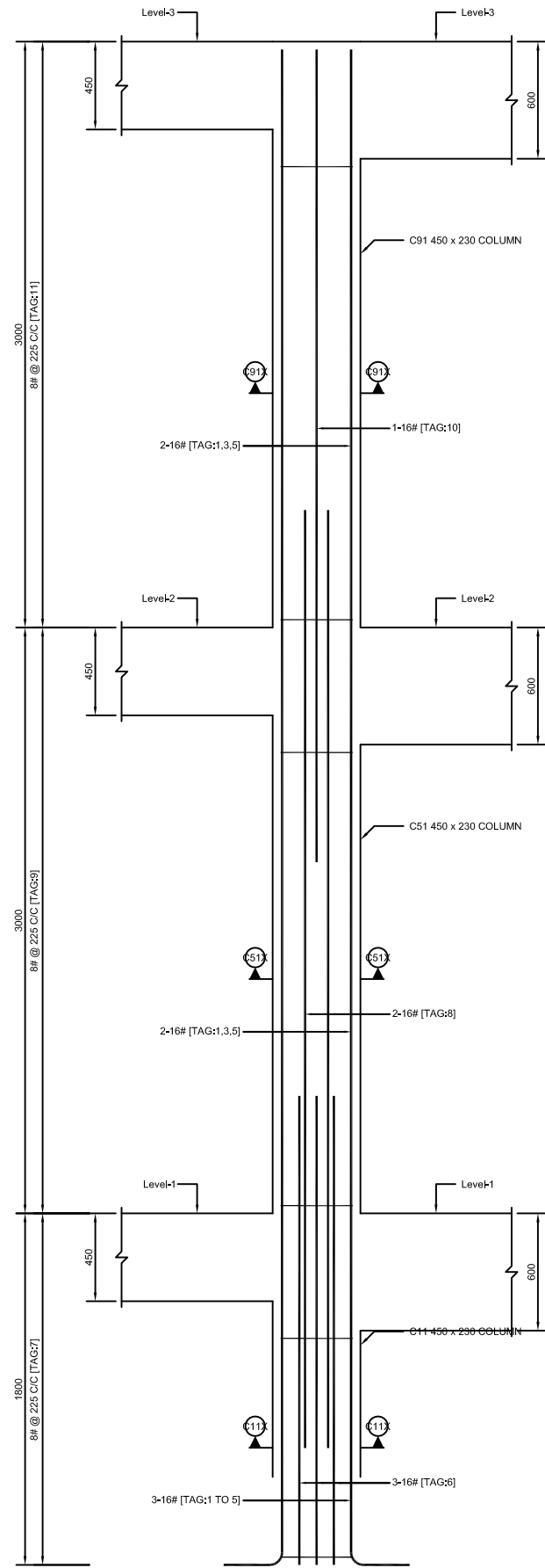
SECTION AT C91X
